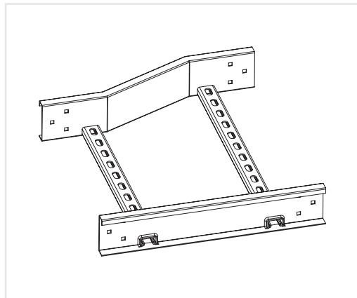
Left hand Offset Reducer KCTL L50 / 100 / 150 . LHR / Width
